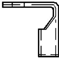
90 Degree Inward Spade
