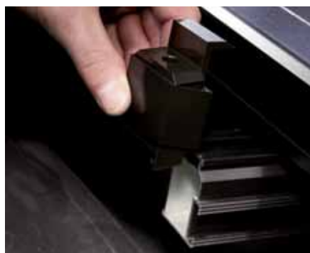
Push the end clamp on the mounting rail
