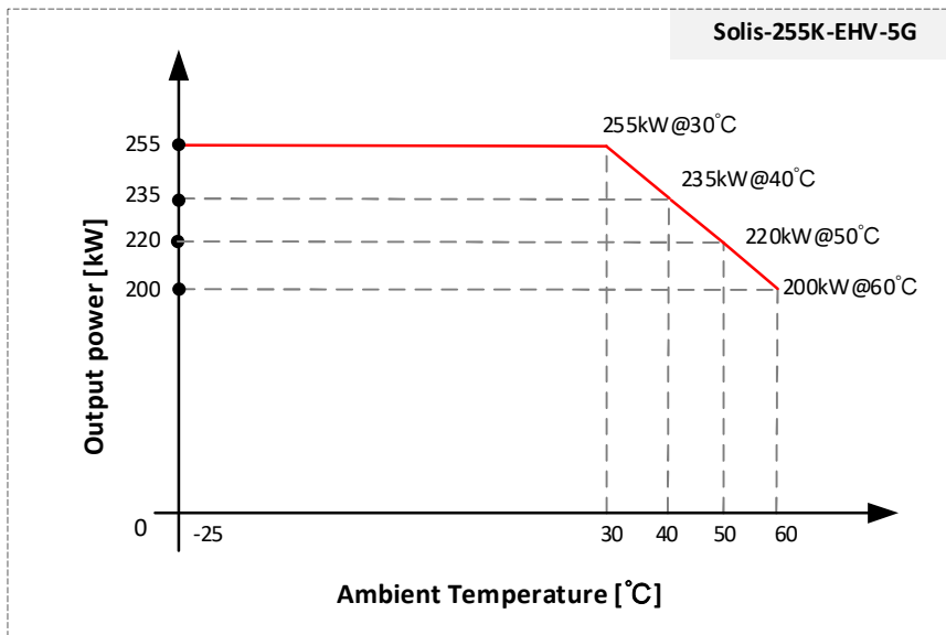
Fig-1: Temperature Derating Curve
