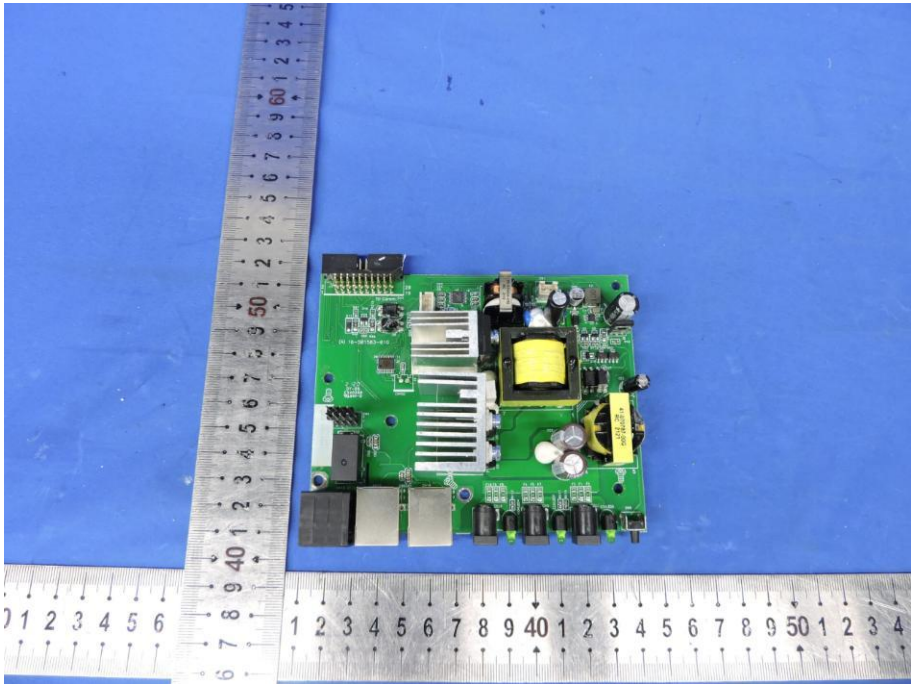
Fig. 22---PCB View
