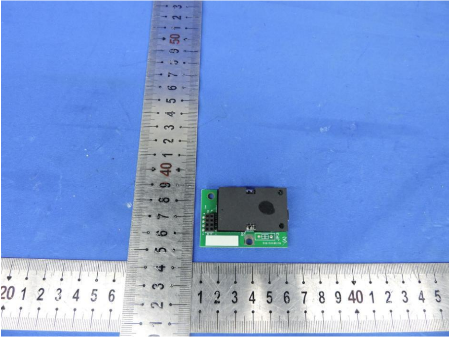
Fig. 26---PCB View
