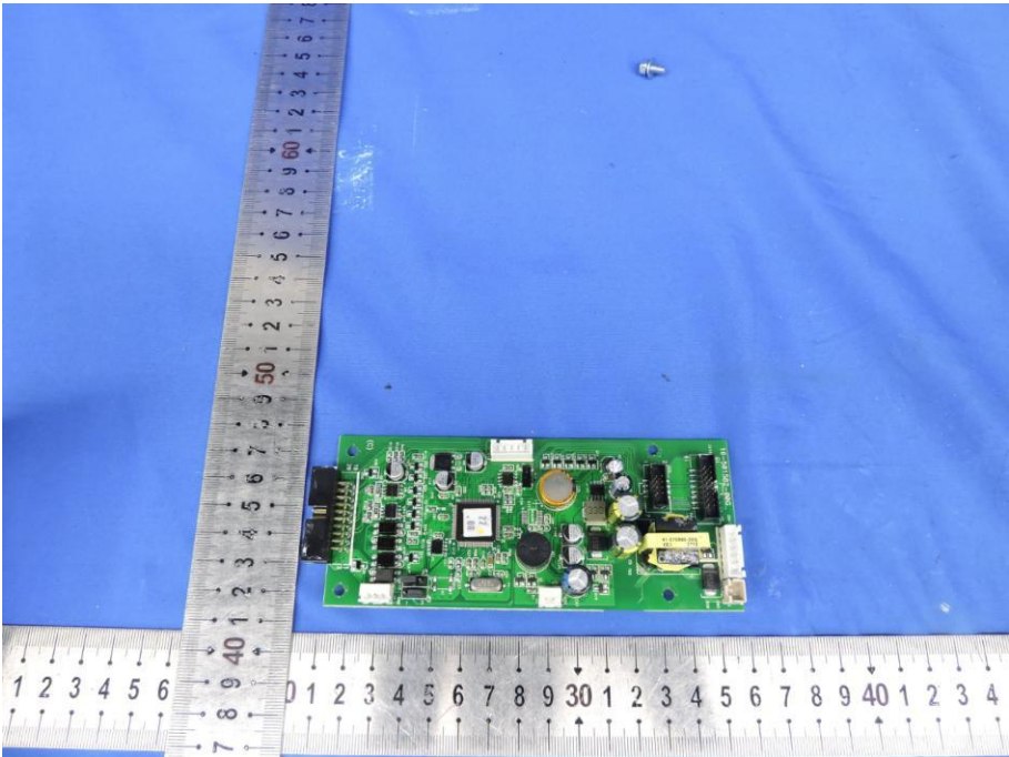
Fig. 10---PCB View
