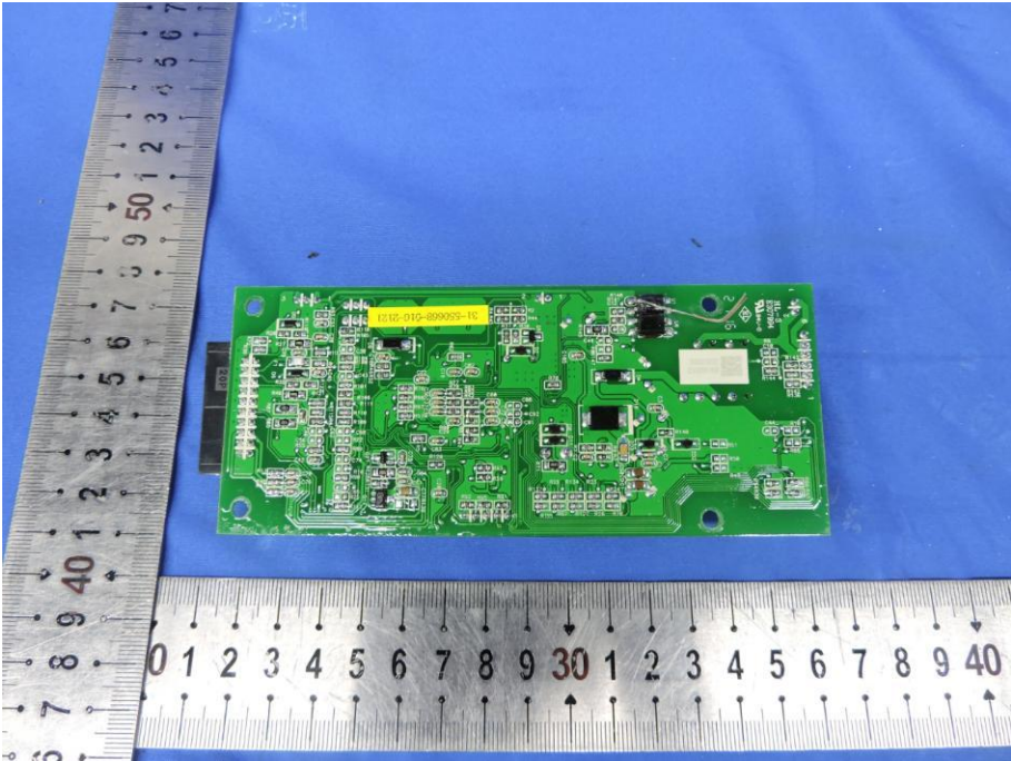
Fig. 11---PCB View
