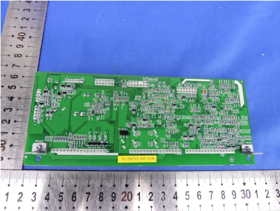
Fig. 25---PCB View
