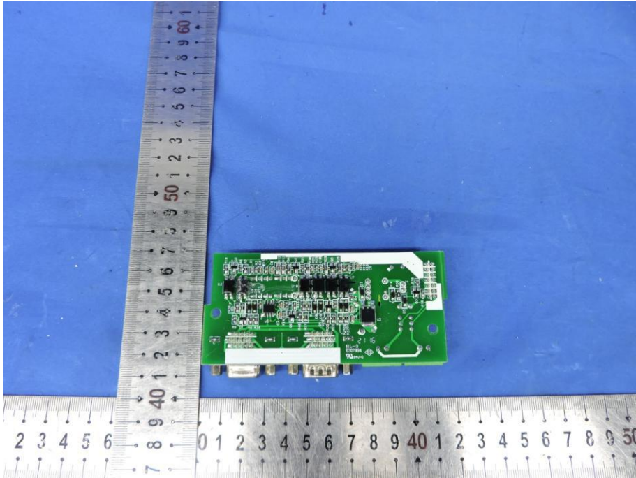
Fig. 21---PCB View
