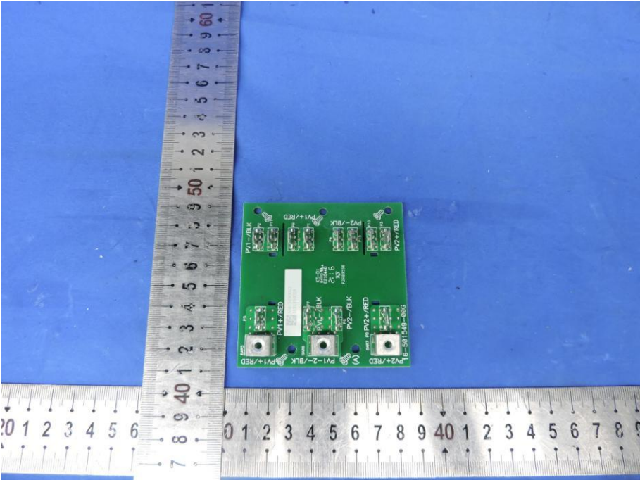
Fig. 18---PCB View
