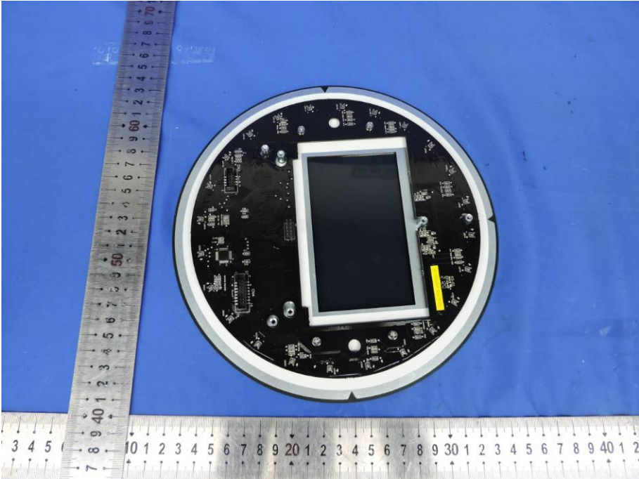
Fig. 30---PCB View
