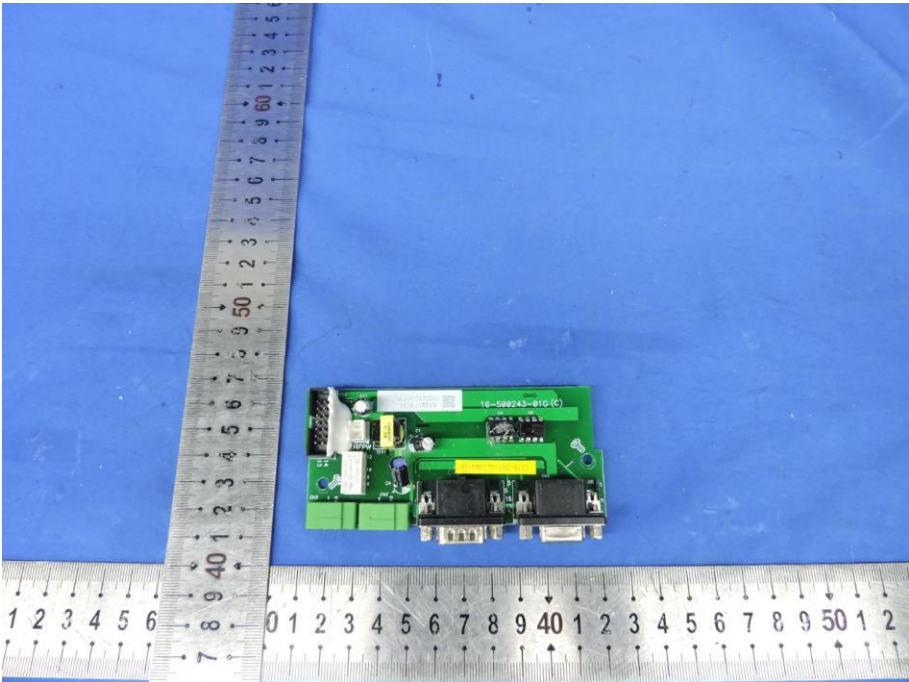
Fig. 20---PCB View
