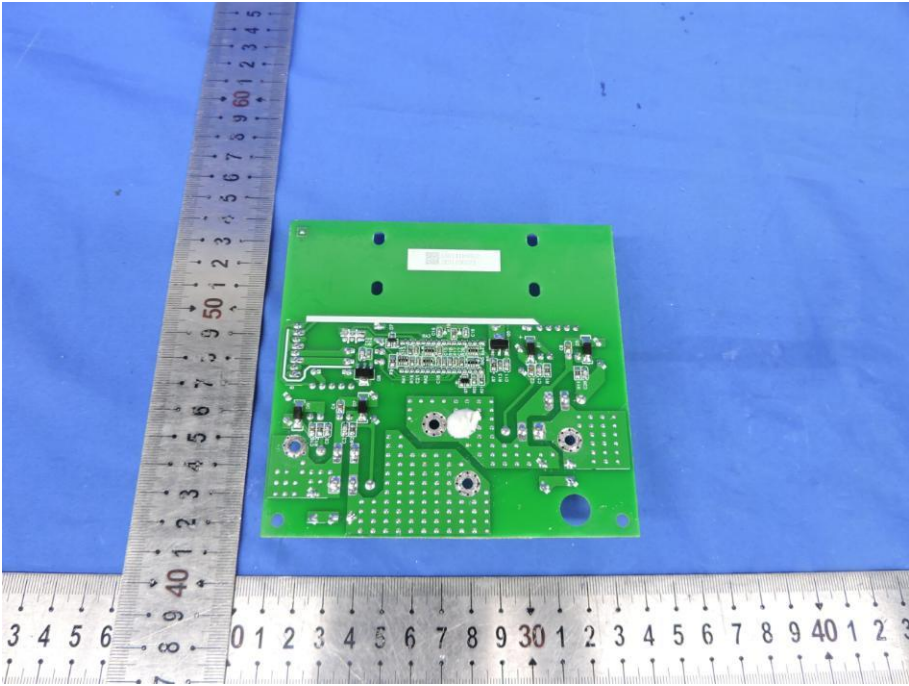
Fig. 17---PCB View
