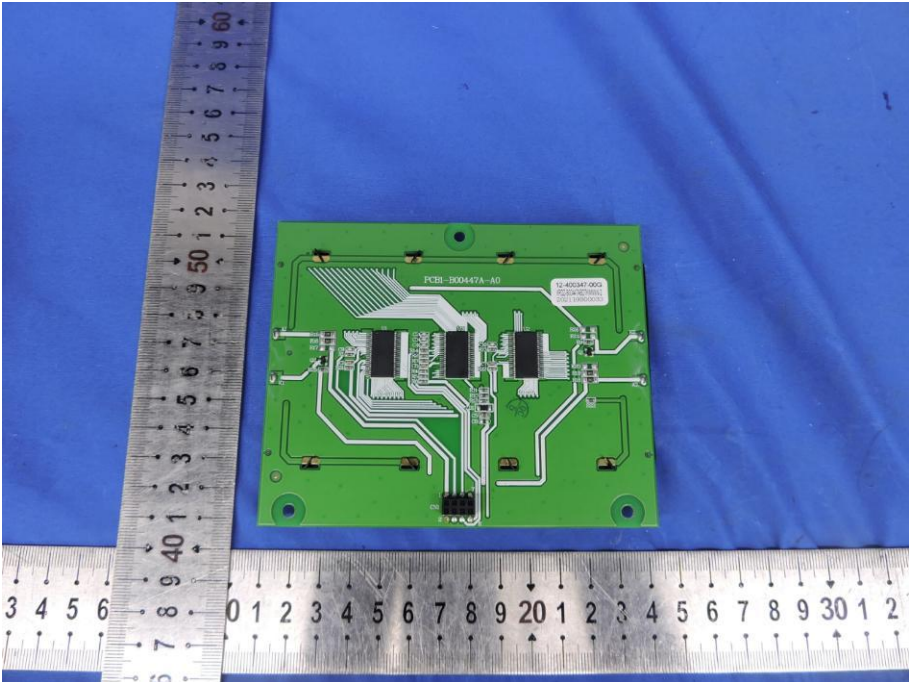
Fig. 29---PCB View
