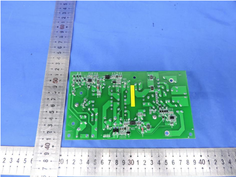
Fig. 15---PCB View
