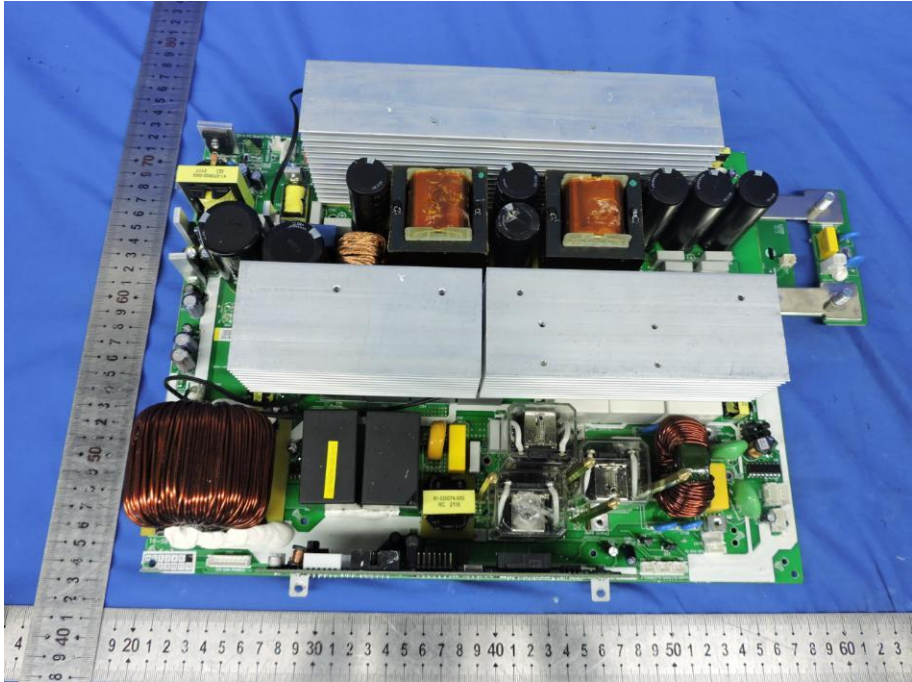
Fig. 8---PCB View
