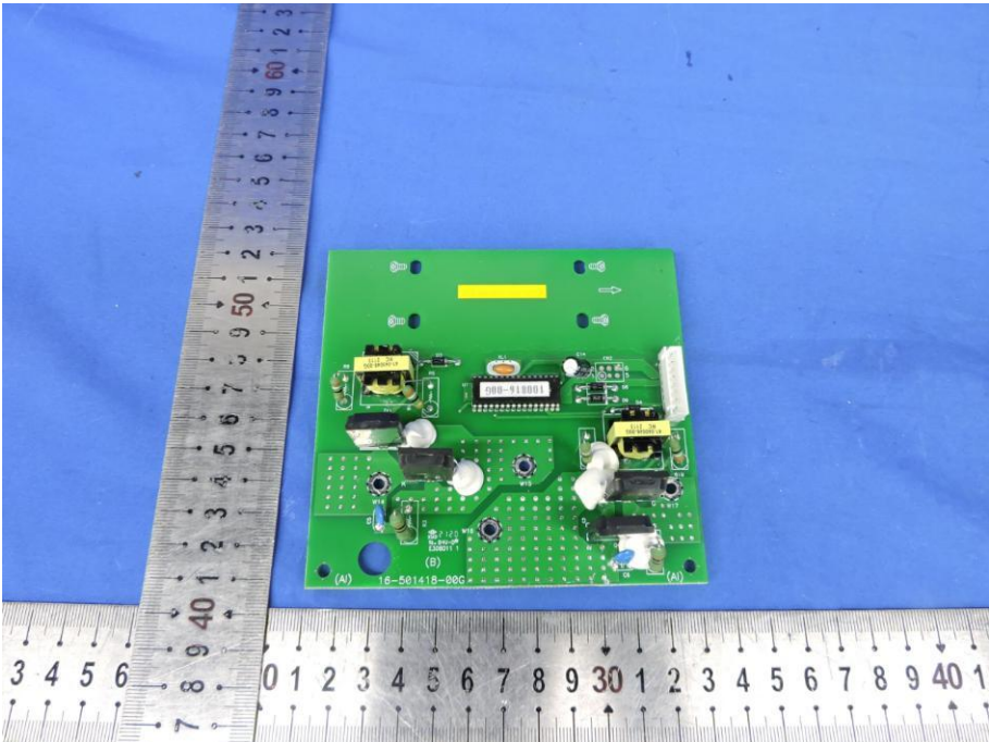
Fig. 16---PCB View
