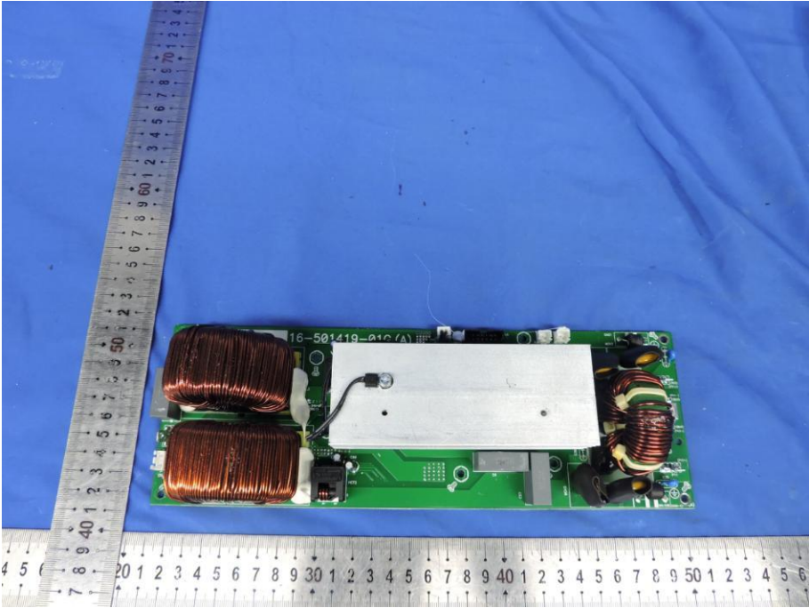
Fig. 12---PCB View
