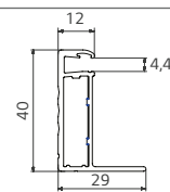
Frame Cross-section
