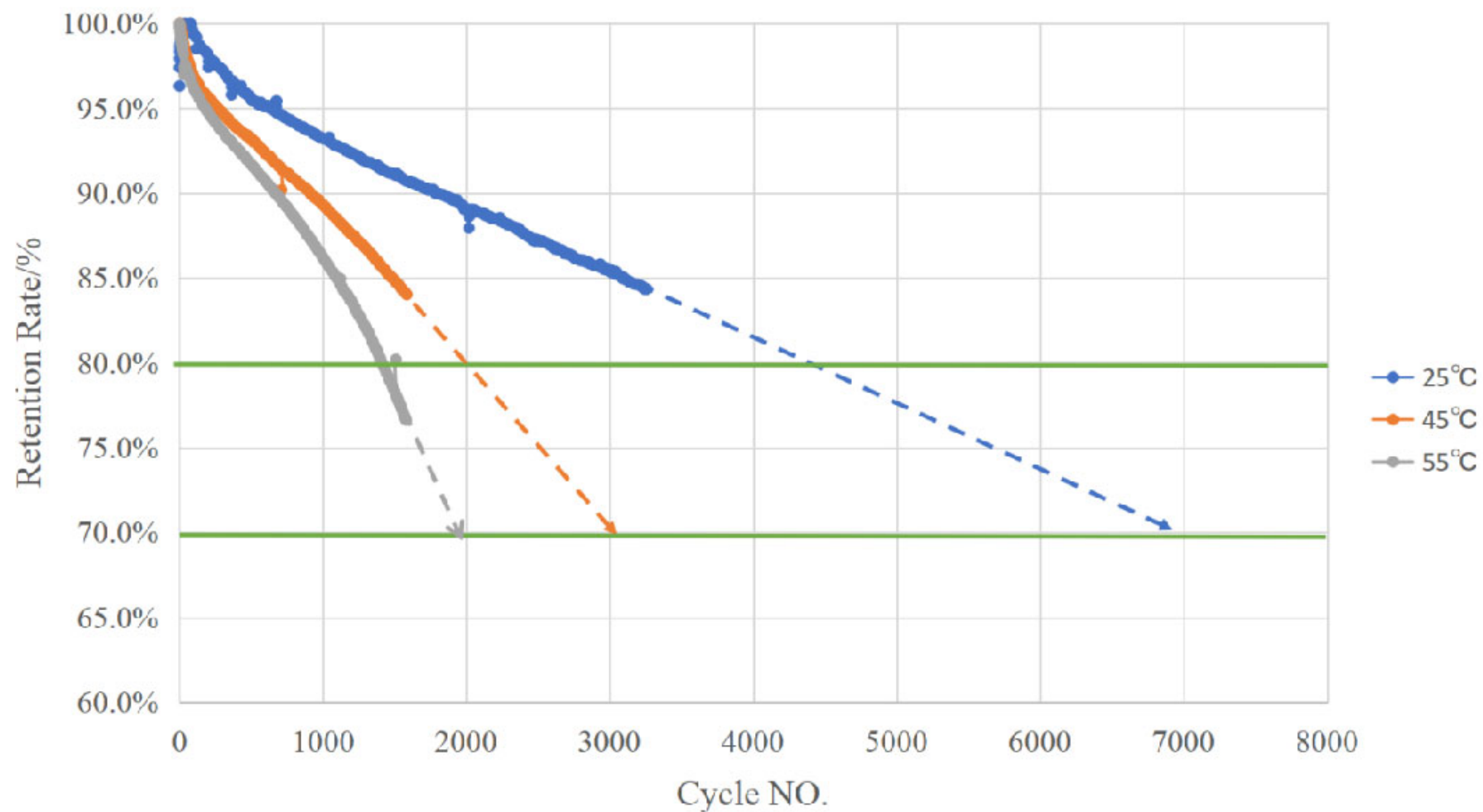
50Ah Cycle Life @ Different Temperature -100%DOD
