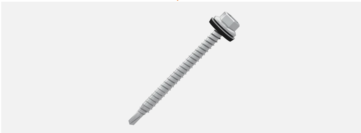
Self-drilling Universal Screw, Buildex 14-11 x 70 Hex Head Zips Climaseal 5 with 16 mm ABW
